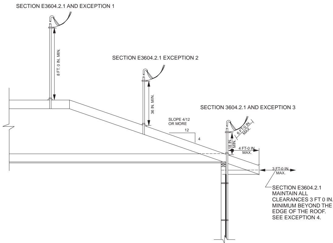
FIGURE E3604.2.1 CLEARANCES FROM ROOFS
