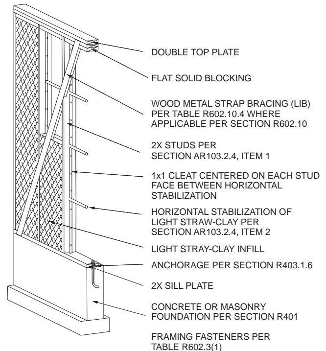
FIGURE AR103.2.4(2) LIGHT STRAW-CLAY WALL SINGLE STUD WIDTH
