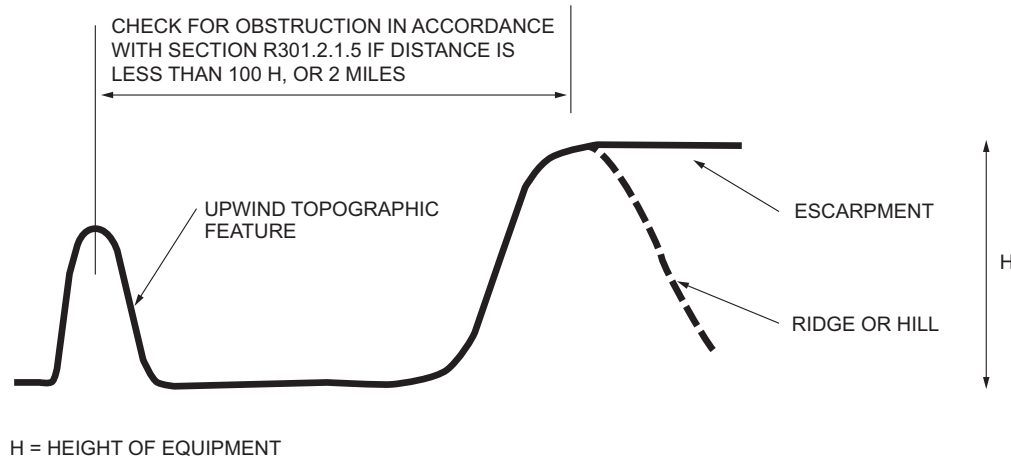
FIGURE R301.2.1.5.1(3) UPWIND OBSTRUCTION
