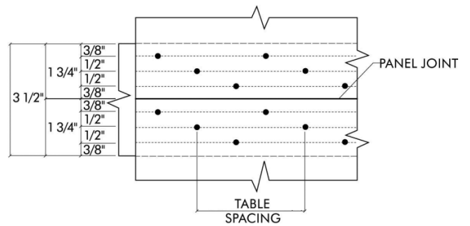
4" NOMINAL—THREE LINES
