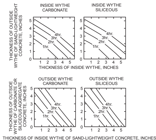
FIGURE 722.2.1.2 FIRE-RESISTANCE RATINGS OF TWO-WYTHE CONCRETE WALLS
