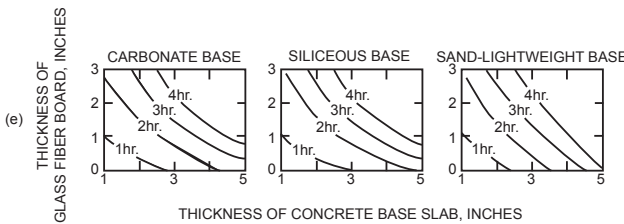
FIGURE 722.2.2.3(2) FIRE-RESISTANCE RATINGS FOR CONCRETE ROOF ASSEMBLIES
