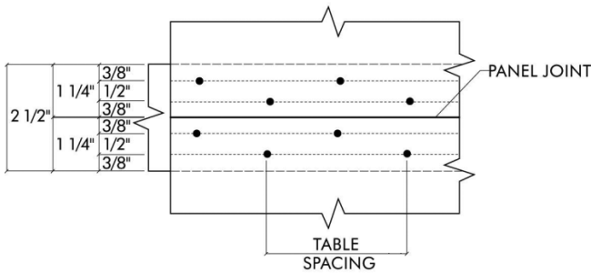
3" NOMINAL—TWO LINES
