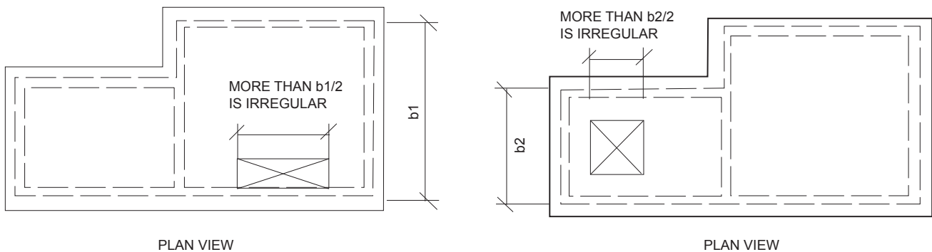
FIGURE 2308.4.1(2) OPENING LIMITATIONS FOR FLOOR AND ROOF DIAPHRAGMS
