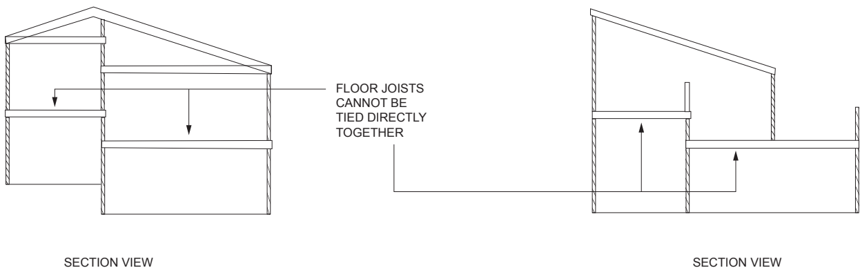
FIGURE 2308.4.2 PORTIONS OF FLOOR LEVEL OFFSET VERTICALLY
